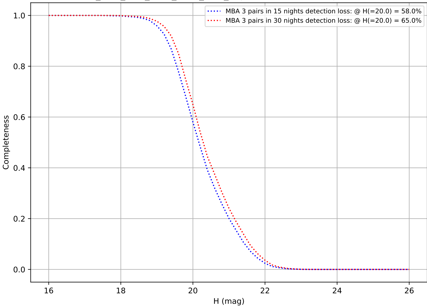
ddf_acor_sf30_lsf40_lsr50_v3.4_10yrs: DifferentialCompleteness
