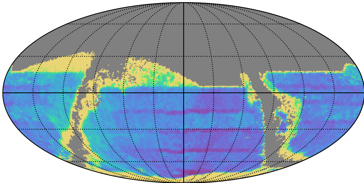
ddf_acor_sf30_ls40_lsr50_v3.4_10yrs : TDC_accuracy
