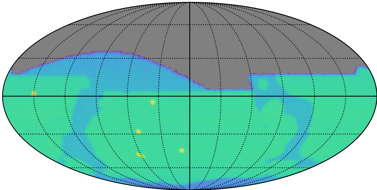
ddf_acor_sf30_lsf40_lsr50_v3.4_10yrs i: SurfaceBrightLimit
