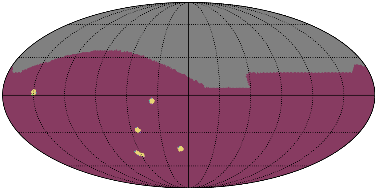
ddf_acor_sf30_lsf40_lsr50_v3.4_10yrs : NumberOfQuickRevisits
