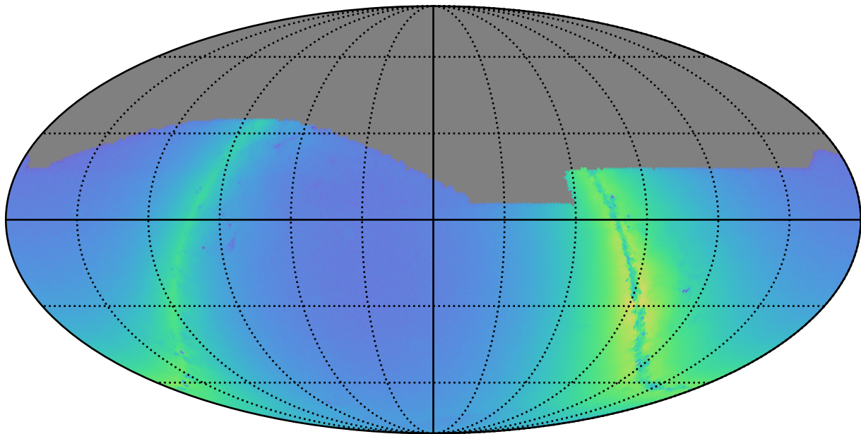
ddf_acor_sf30_lsf40_lsr50_v3.4_10yrs r: Nstars_no_crowding
