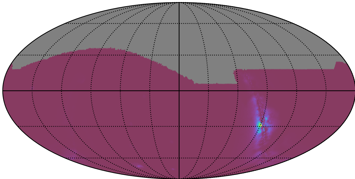
ddf_acor_sf30_lsf40_lsr50_v3.4_10yrs : NlcPoints
