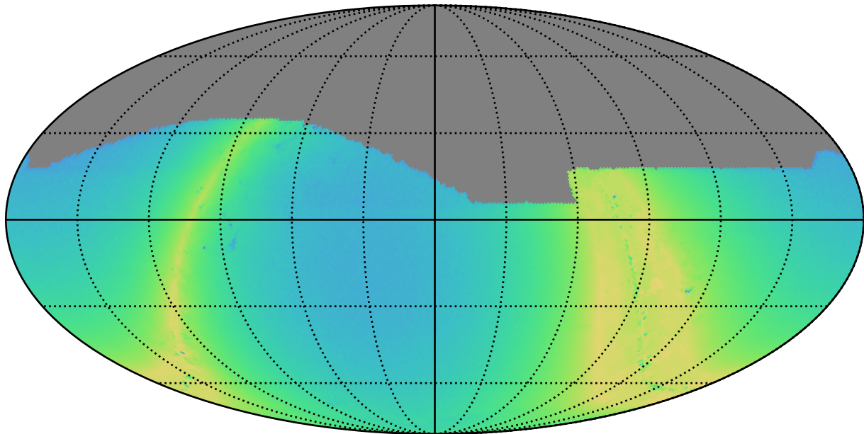
ddf_acor_sf30_lsf40_lsr50_v3.4_10yrs i: N stars to Precision 0.20
