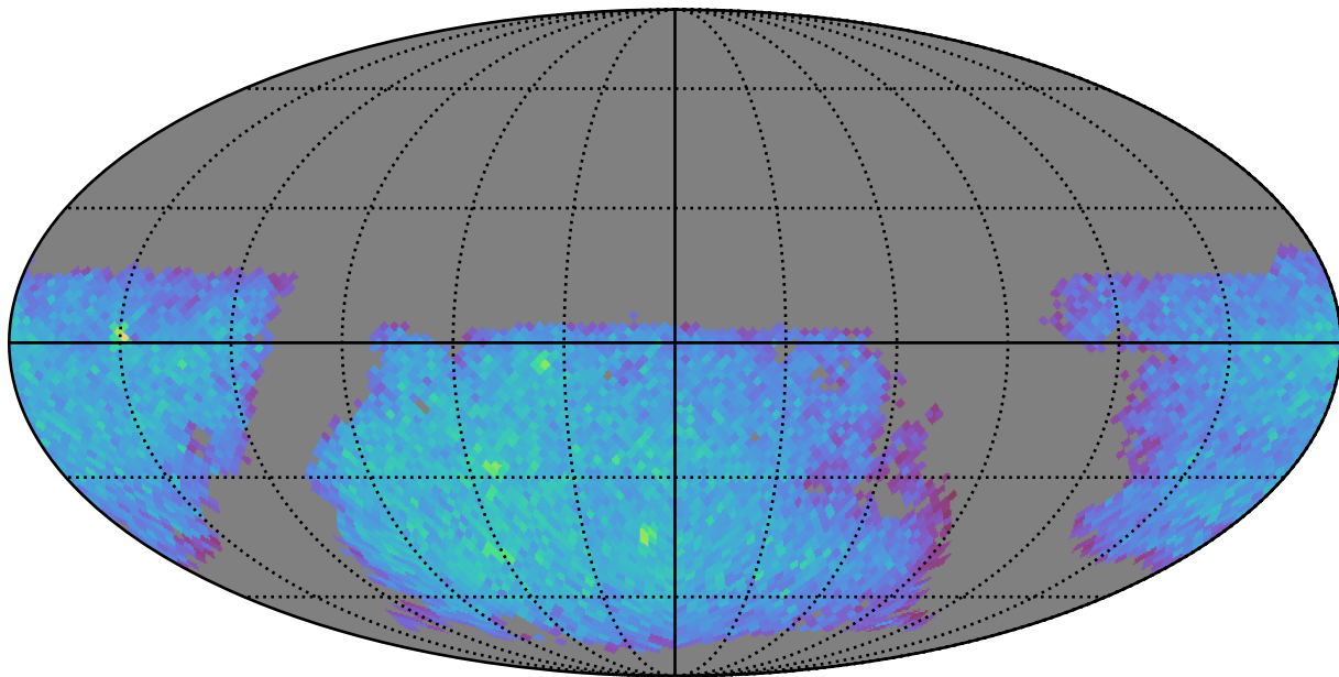
ddf_acor_sf30_lsf40_lsr50_v3.4_10yrs gi: LVDwarfs
