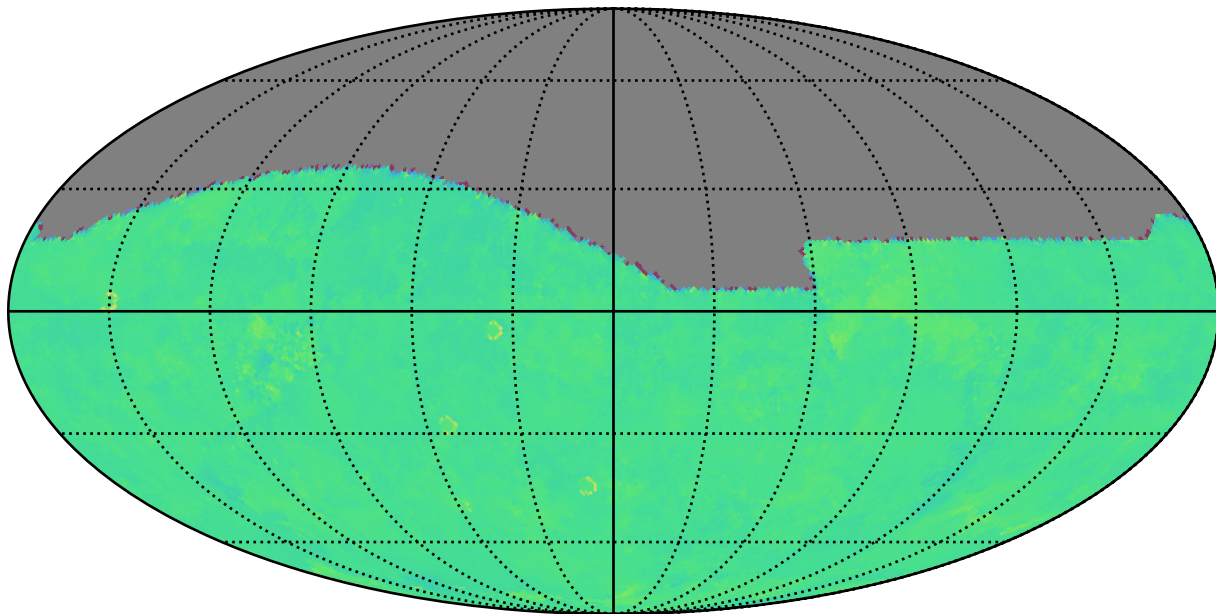
ddf_acor_sf30_lsf40_lsr50_v3.4_10yrs g: Kuiper rotTelPos
