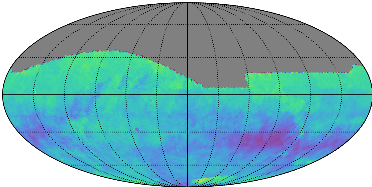
ddf_acor_sf30_lsf40_lsr50_v3.4_10yrs r: Kuiper rotSkyPos
