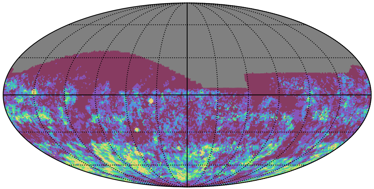
ddf_acor_sf30_lsf40_lsr50_v3.4_10yrs r band: Gaps_3hr
