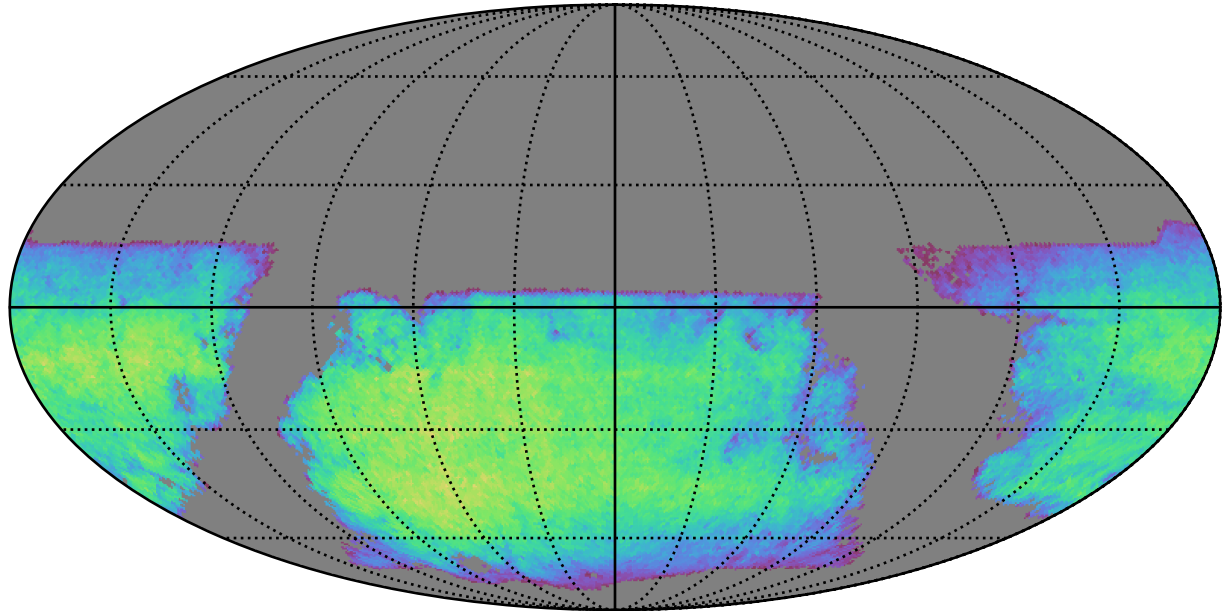
ddf_acor_sf30_lsf40_lsr50_v3.4_10yrs i band non-DD year 10: ExgalM5WithCuts
