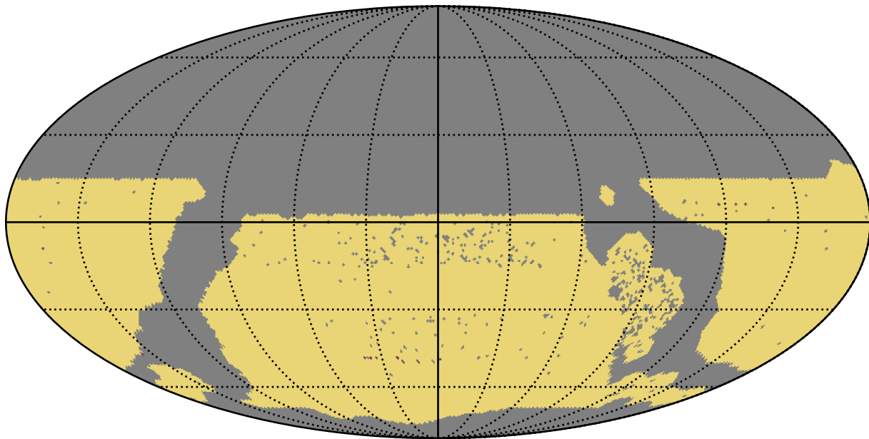
ddf_acor_sf30_lsf40_lsr50_v3.4_10yrs WFD: RapidRevisits
