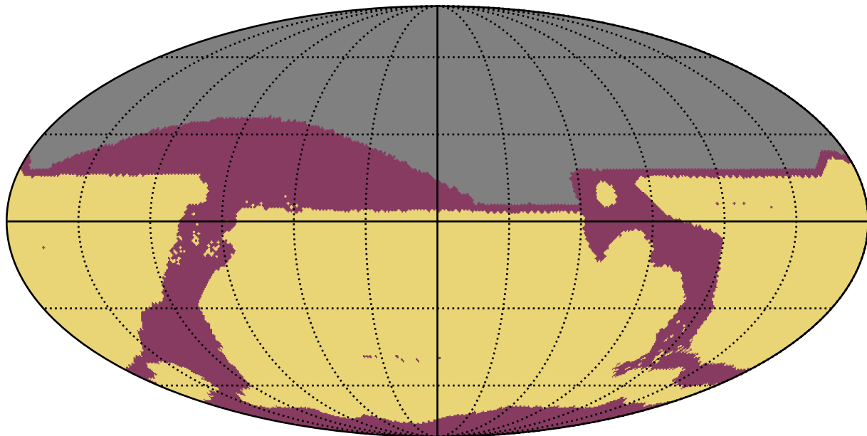
ddf_acor_sf30_lsf40_lsr50_v3.4_10yrs All sky: RapidRevisits
