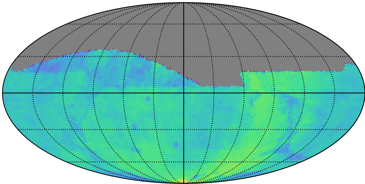
ddf_acor_sf30_lsf40_lsr50_v3.4_10yrs All sky: Parallax Coverage @ 24.0
