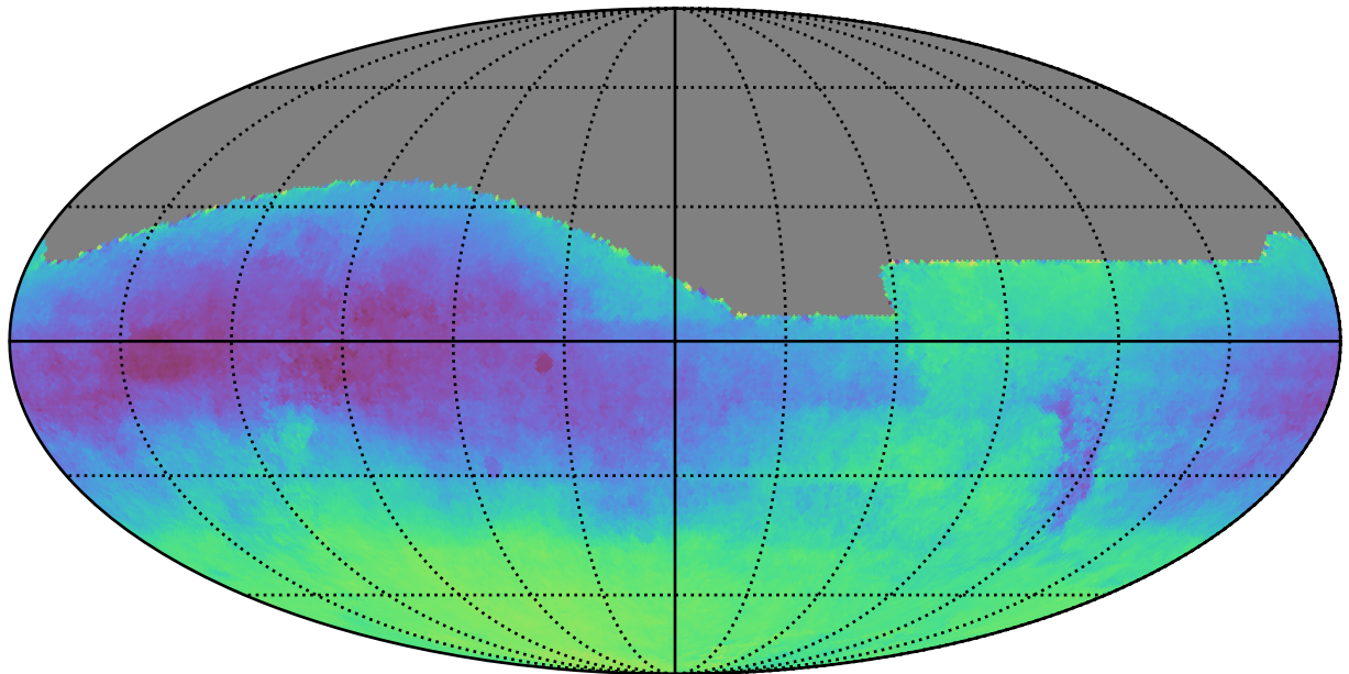
ddf_acor_sf30_lsf40_lsr50_v3.4_10yrs All sky: Parallax-DCR degeneracy @ 22.4
