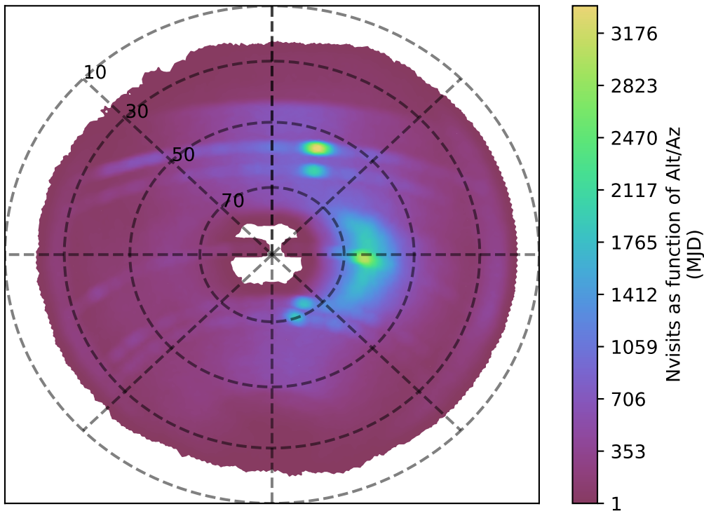
ddf_acor_sf30_lsf40_lsr50_v3.4_10yrs z band: Nvisits as function of Alt/Az
