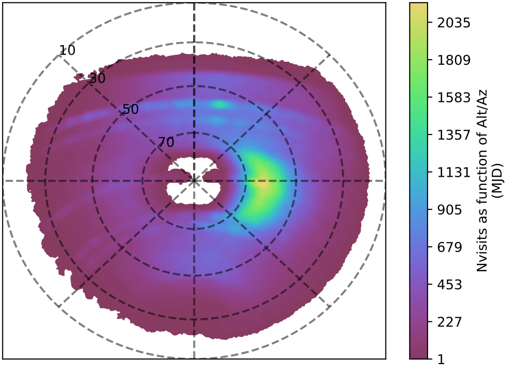
ddf_acor_sf30_lsf40_lsr50_v3.4_10yrs y band: Nvisits as function of Alt/Az
