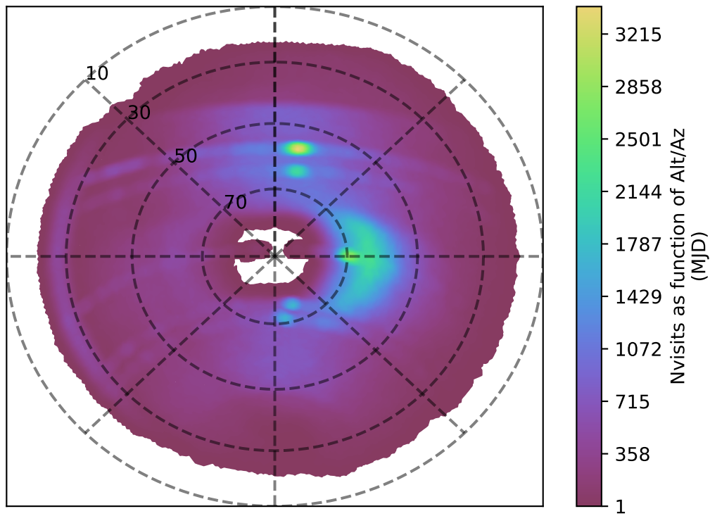
ddf_acor_sf30_lsf40_lsr50_v3.4_10yrs r band: Nvisits as function of Alt/Az
