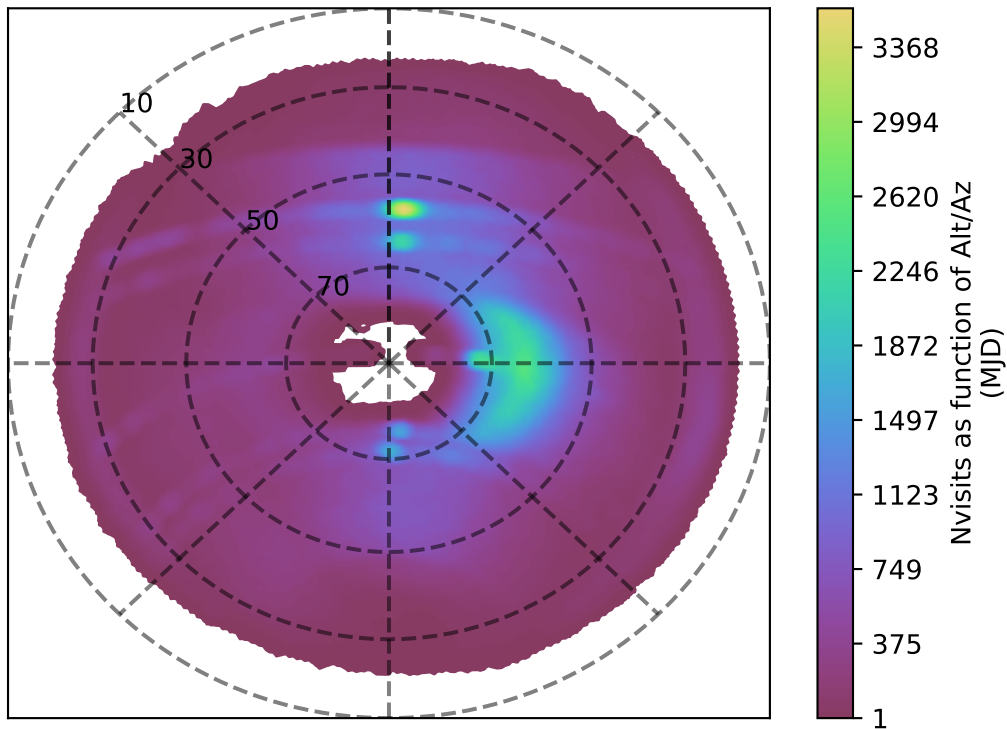
ddf_acor_sf30_lsf40_lsr50_v3.4_10yrs i band: Nvisits as function of Alt/Az
