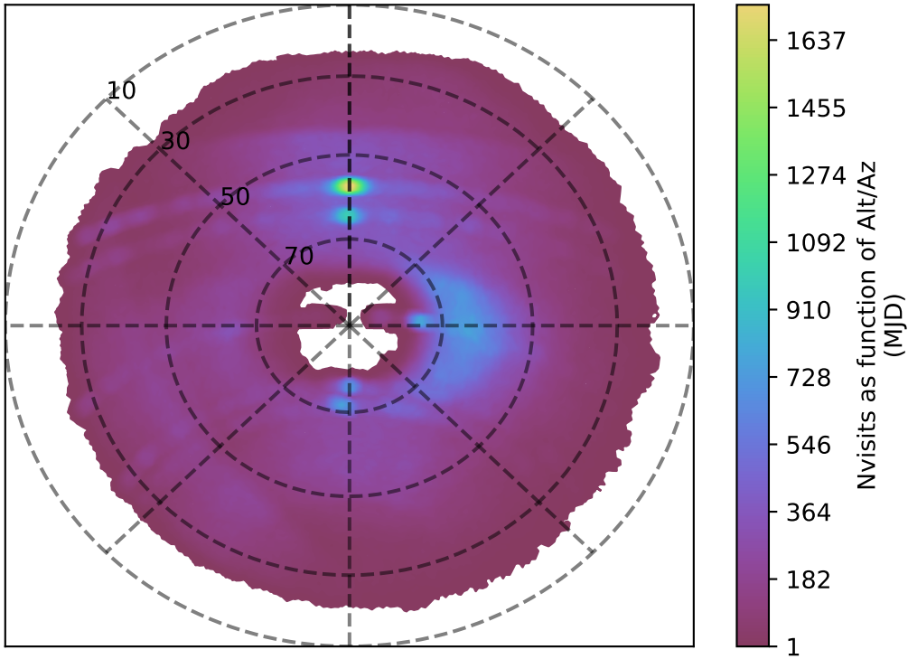
ddf_acor_sf30_lsf40_lsr50_v3.4_10yrs g band: Nvisits as function of Alt/Az
