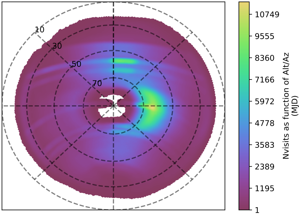
ddf_acor_sf30_ls40_lsr50_v3.4_10yrs all bands: Nvisits as function of Alt/Az
