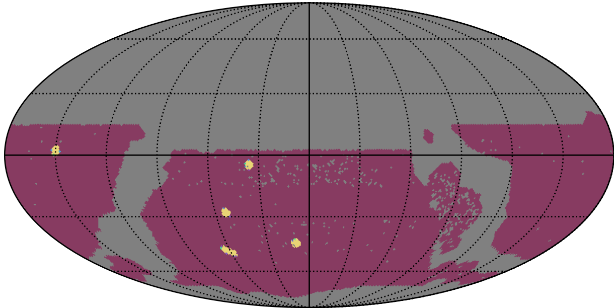
ddf_acor_sf30_lsf40_lsr50_v3.4_10yrs WFD: NumberOfQuickRevisits
