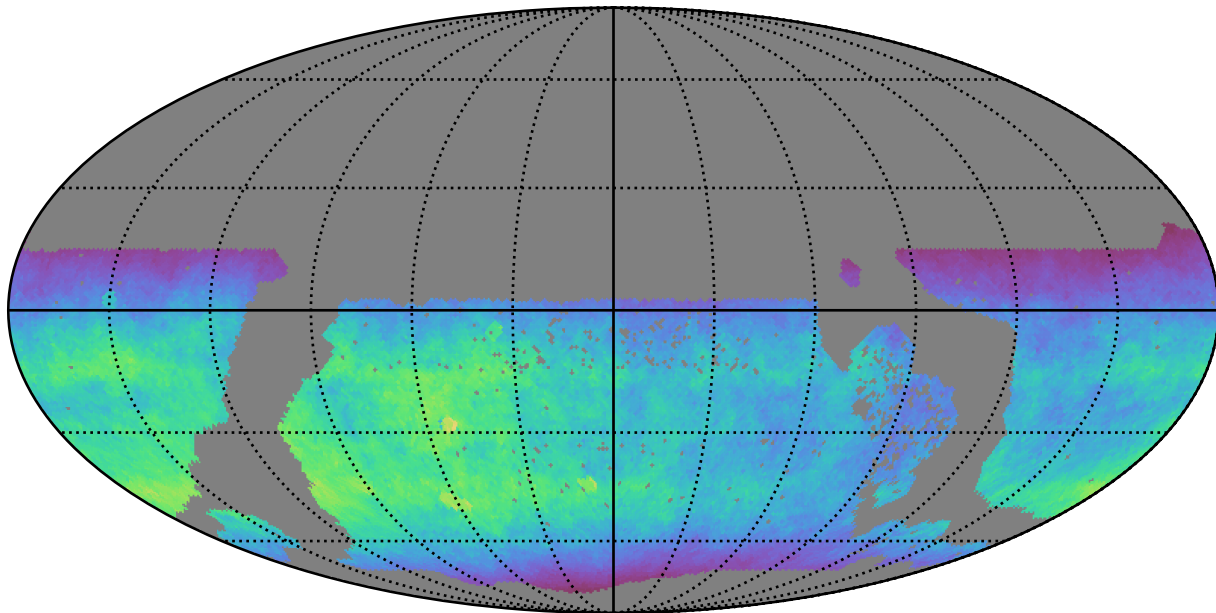
ddf_acor_sf30_lsf40_lsr50_v3.4_10yrs WFD y band: Normalized Teff
