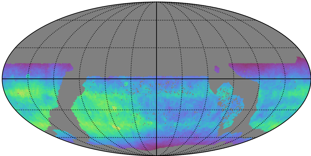
ddf_acor_sf30_lsf40_lsr50_v3.4_10yrs WFD i band: Normalized Teff
