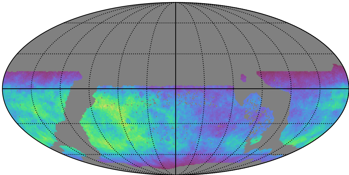
ddf_acor_sf30_lsf40_lsr50_v3.4_10yrs WFD g band: Normalized Teff
