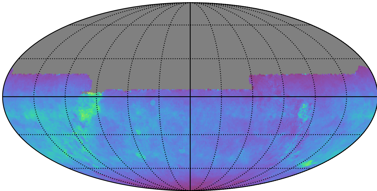
ddf_acor_sf30_lsf40_lsr50_v3.4_10yrs All sky u band: Normalized Teff
