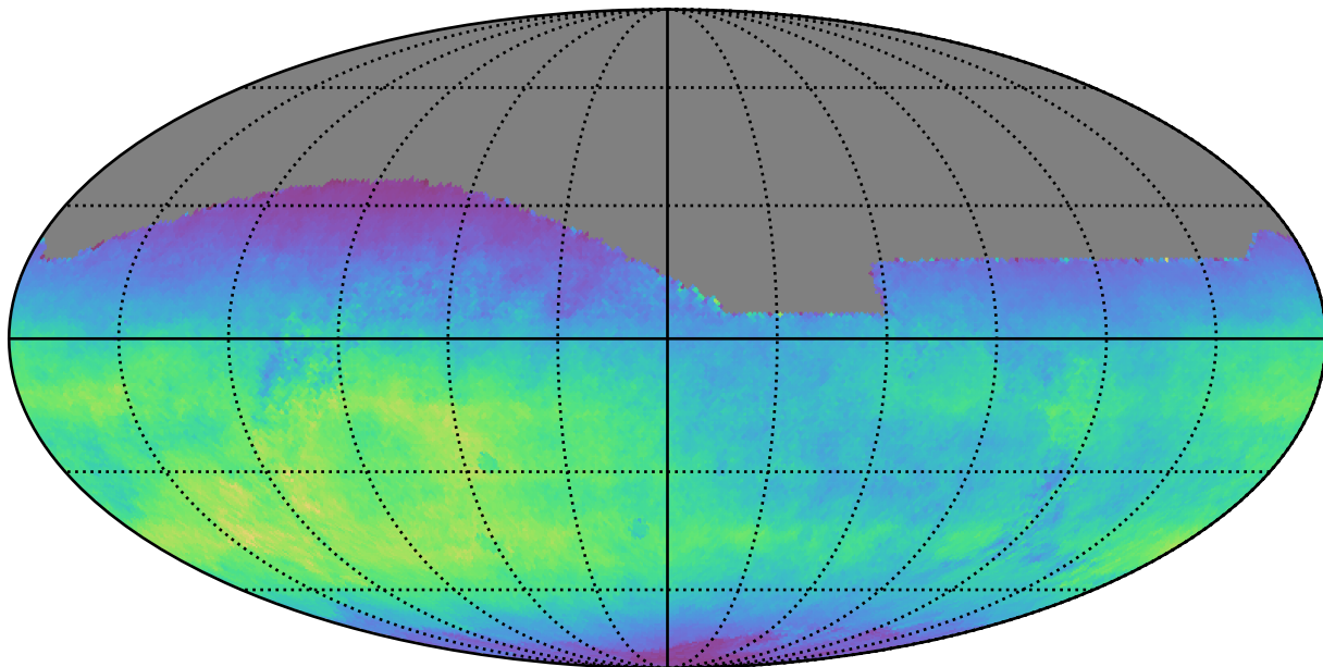
ddf_acor_sf30_lsf40_lsr50_v3.4_10yrs All sky r band: Normalized Teff
