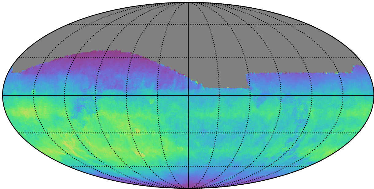
ddf_acor_sf30_lsf40_lsr50_v3.4_10yrs All sky i band: Normalized Teff
