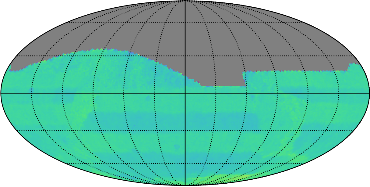
ddf_acor_sf30_lsf40_lsr50_v3.4_10yrs All sky: Normalized Proper Motion Uncert @ 20.5
