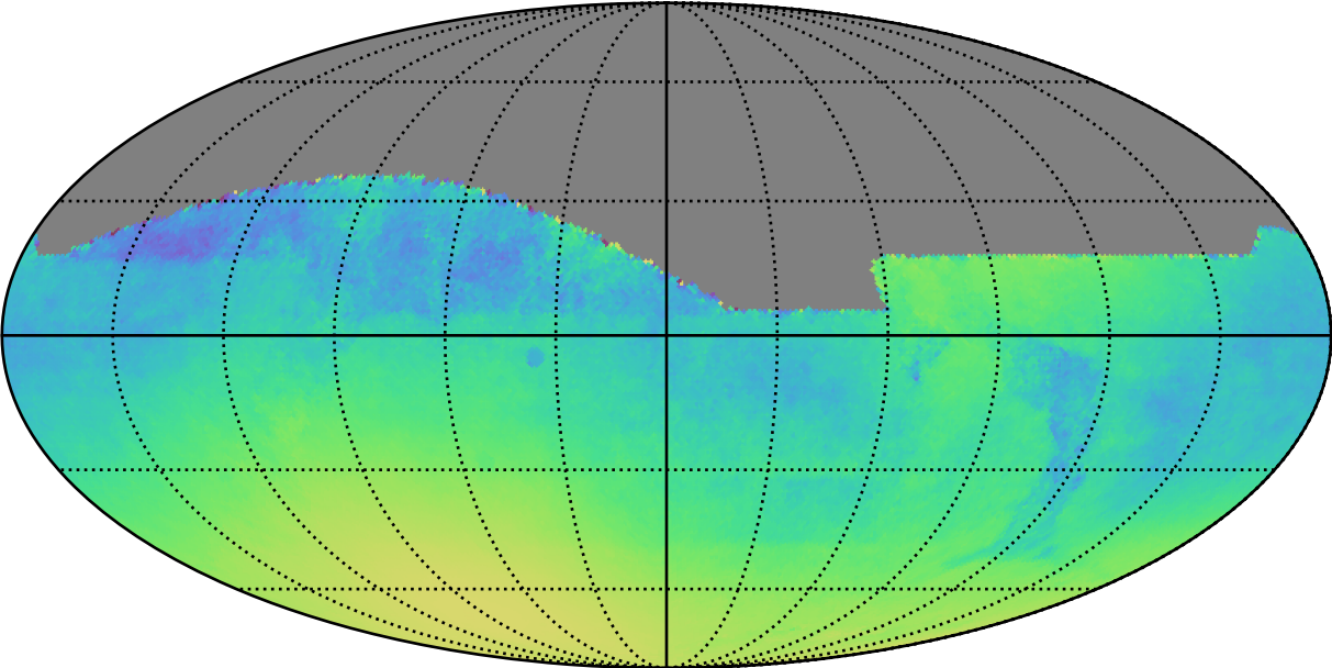
ddf_acor_sf30_lsf40_lsr50_v3.4_10yrs All sky: Normalized Parallax Uncert @ 24.0
