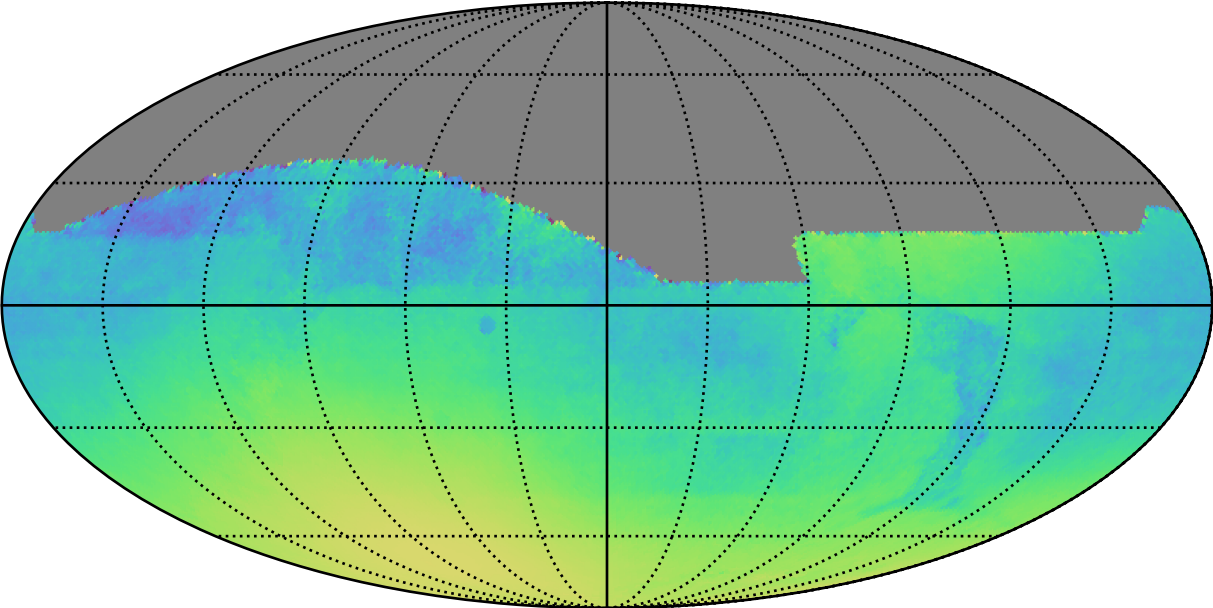
ddf_acor_sf30_lsf40_lsr50_v3.4_10yrs All sky: Normalized Parallax Uncert @ 22.4
