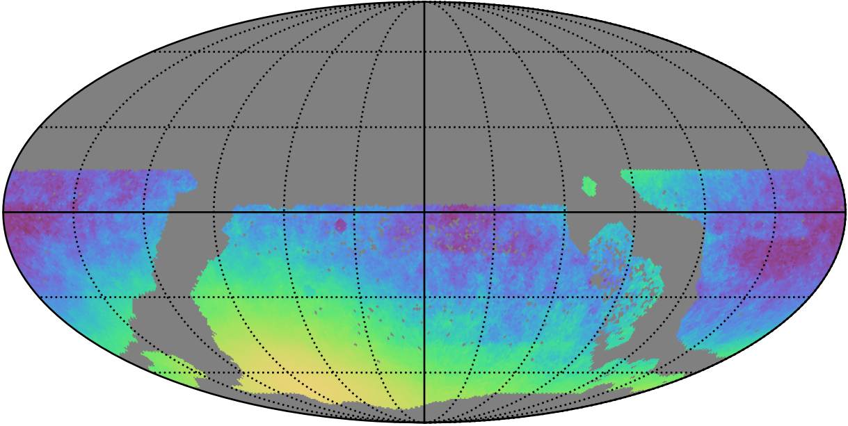
ddf_acor_sf30_lsf40_lsr50_v3.4_10yrs WFD y band only: Normalized Parallax Uncert @ 21.3
