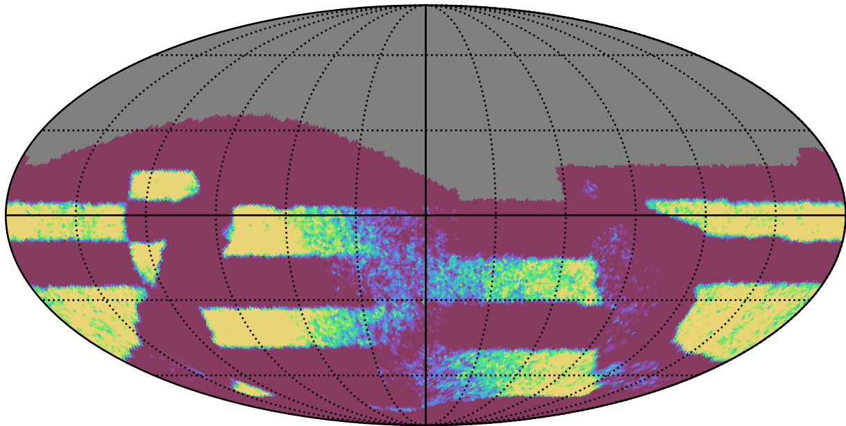
ddf_acor_sf30_lsf40_lsr50_v3.4_10yrs Yr 3-4 all bands: NVisits
