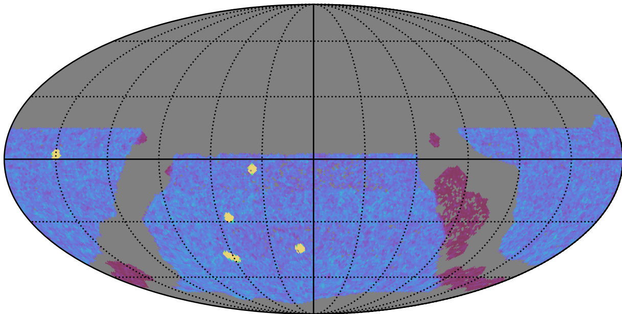
ddf_acor_sf30_lsf40_lsr50_v3.4_10yrs WFD y band: NVisits
