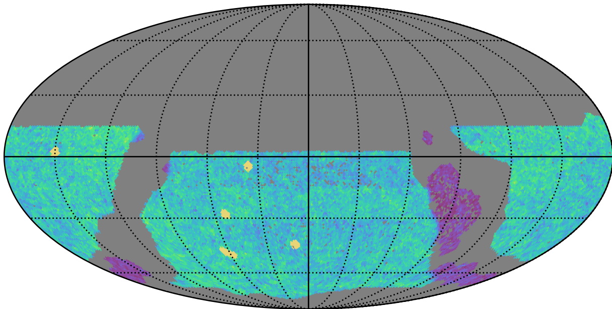
ddf_acor_sf30_lsf40_lsr50_v3.4_10yrs WFD u band: NVisits
