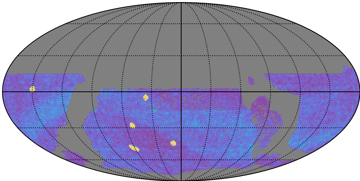
ddf_acor_sf30_lsf40_lsr50_v3.4_10yrs WFD all bands: NVisits
