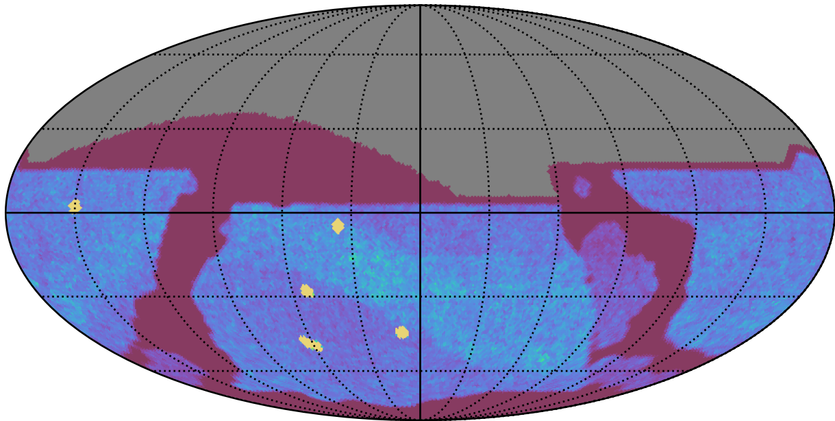
ddf_acor_sf30_lsf40_lsr50_v3.4_10yrs All sky z band: NVisits
