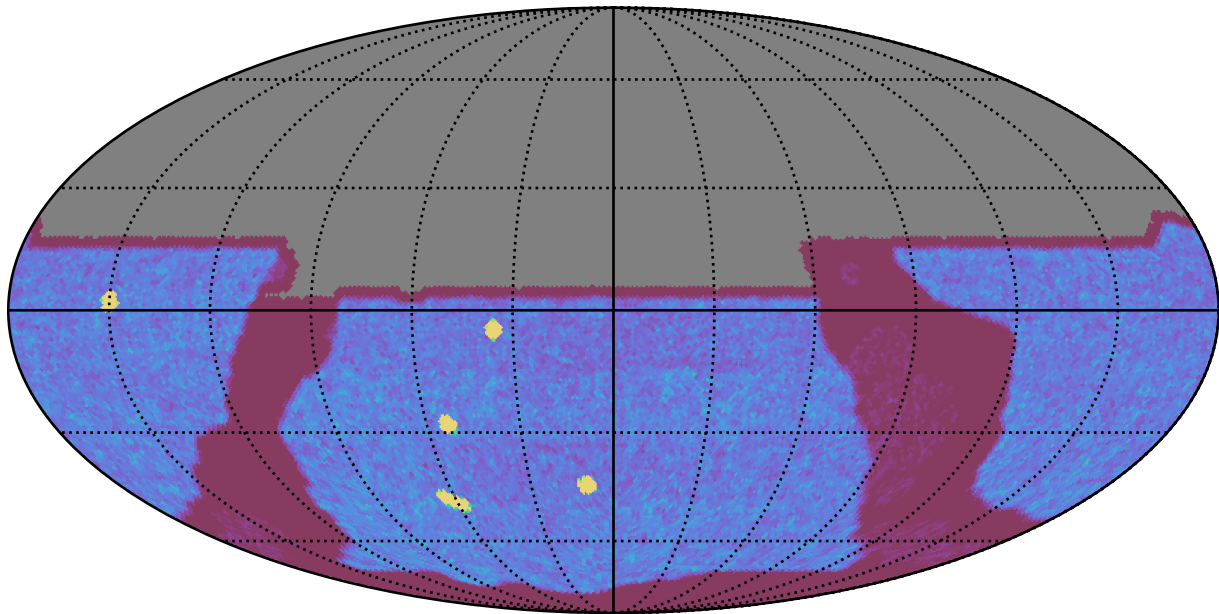
ddf_acor_sf30_lsf40_lsr50_v3.4_10yrs All sky y band: NVisits
