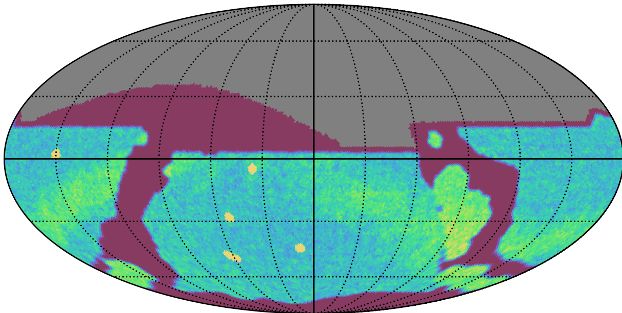
ddf_acor_sf30_lsf40_lsr50_v3.4_10yrs All sky r band: NVisits
