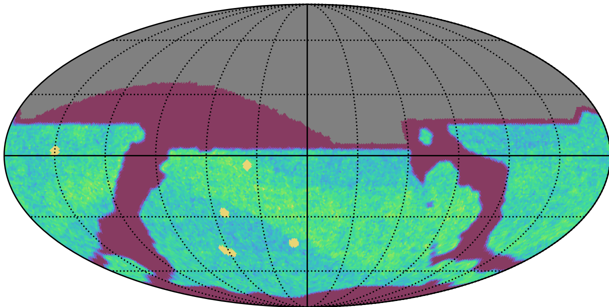
ddf_acor_sf30_lsf40_lsr50_v3.4_10yrs All sky i band: NVisits
