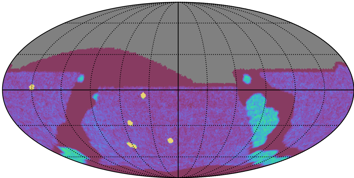
ddf_acor_sf30_lsf40_lsr50_v3.4_10yrs All sky g band: NVisits
