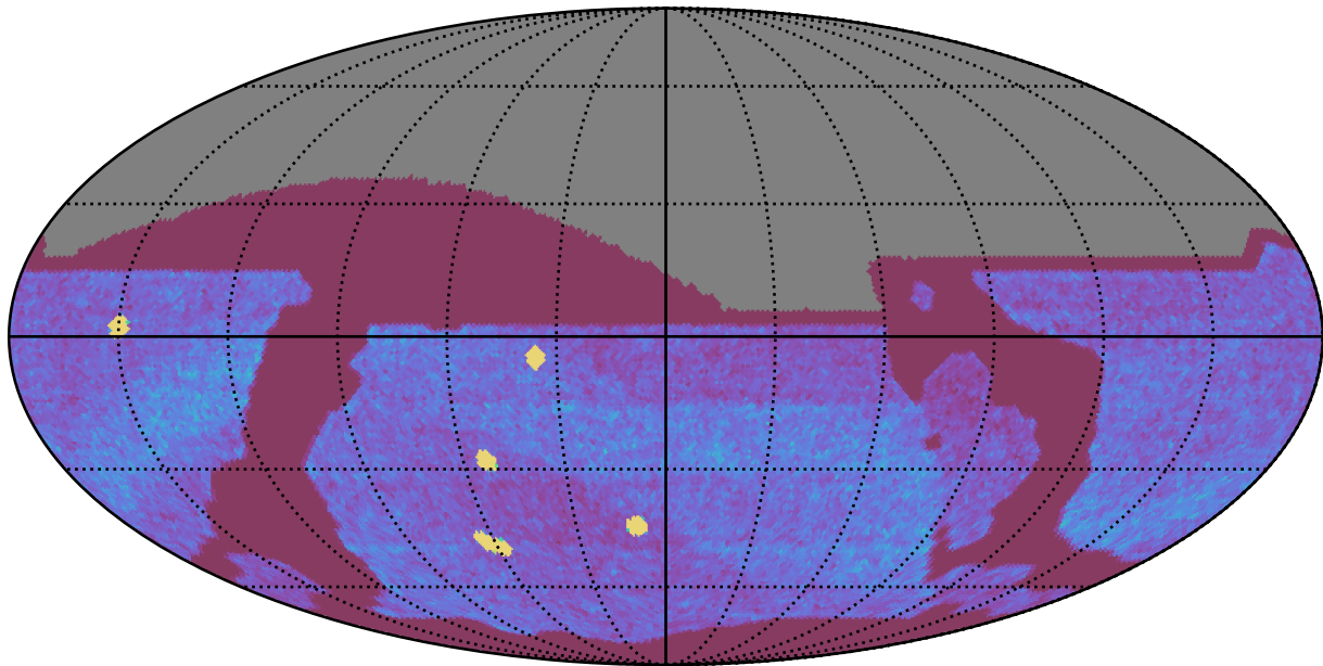
ddf_acor_sf30_lsf40_lsr50_v3.4_10yrs All sky all bands: NVisits
