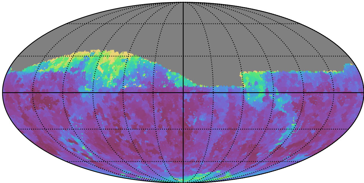
ddf_acor_sf30_lsf40_lsr50_v3.4_10yrs Yr 1 z band: Min seeingEff
