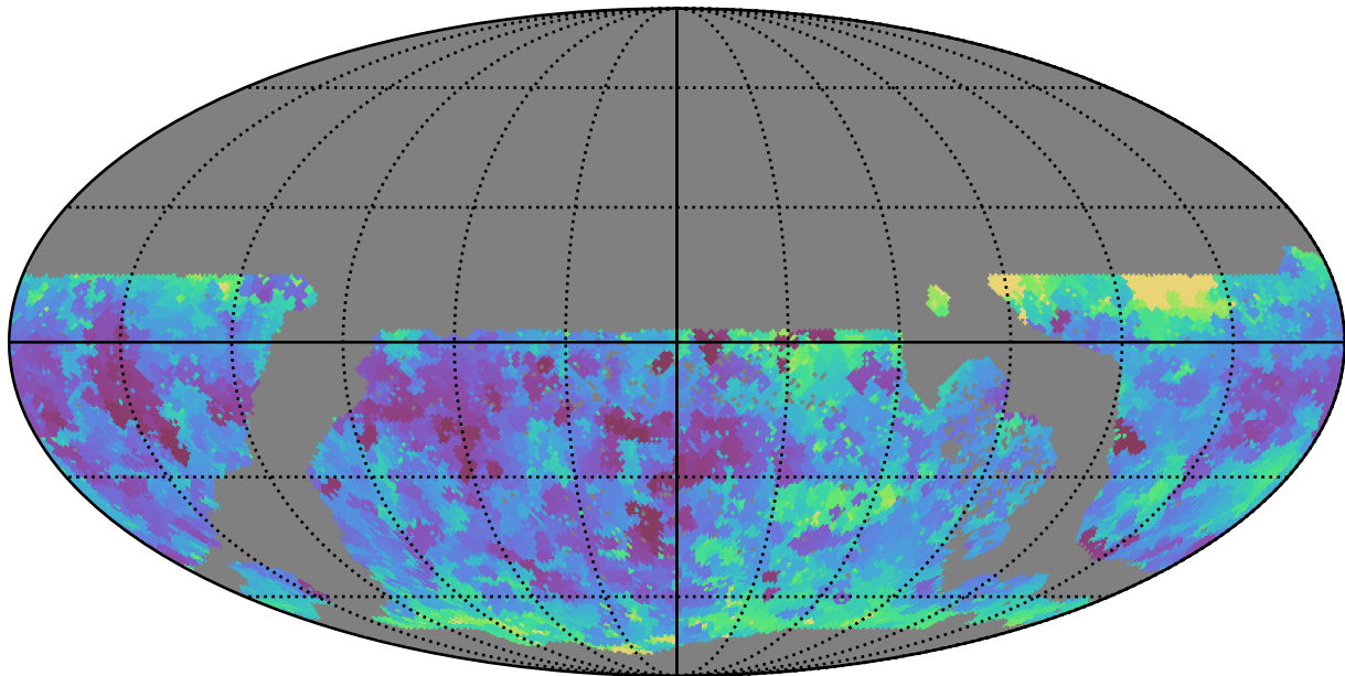
ddf_acor_sf30_lsf40_lsr50_v3.4_10yrs WFD g band: Min seeingEff
