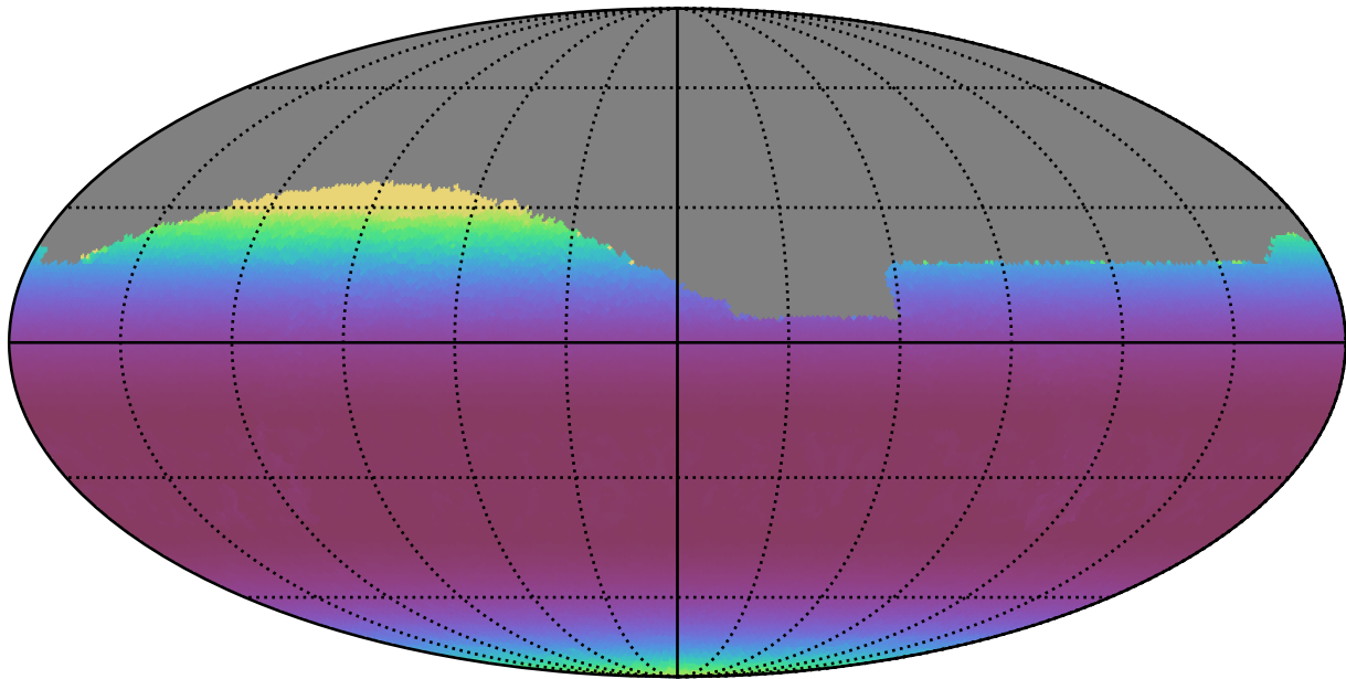
ddf_acor_sf30_lsf40_lsr50_v3.4_10yrs Yr 1 all bands: Min airmass
