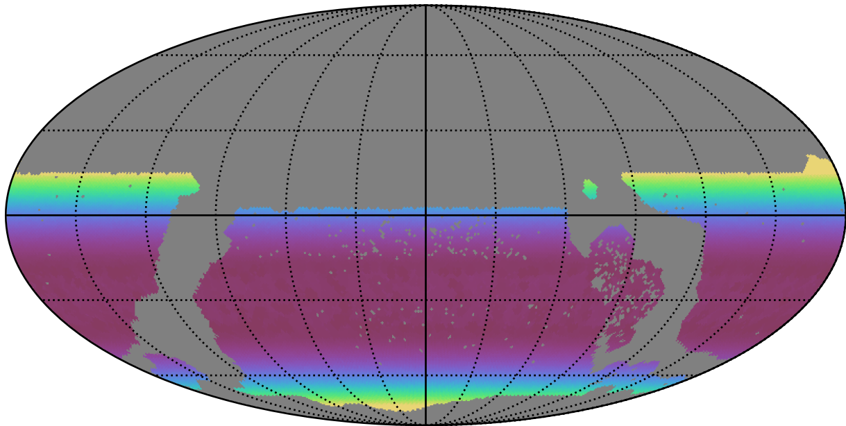
ddf_acor_sf30_lsf40_lsr50_v3.4_10yrs WFD all bands: Min airmass
