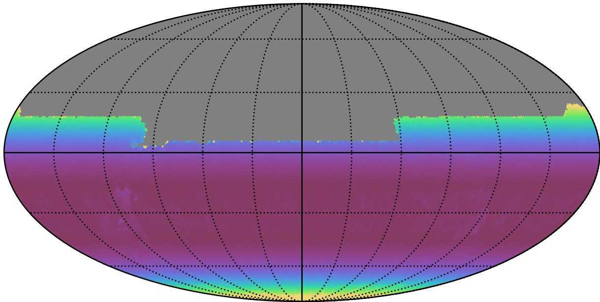
ddf_acor_sf30_lsf40_lsr50_v3.4_10yrs All sky y band: Min airmass
