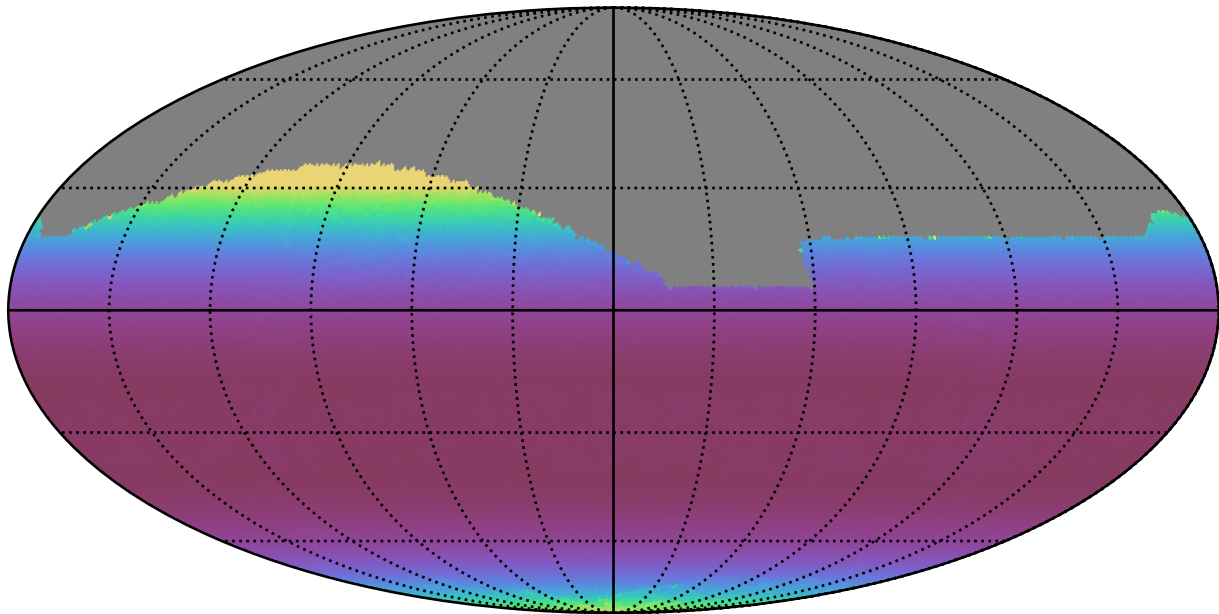
ddf_acor_sf30_lsf40_lsr50_v3.4_10yrs All sky r band: Min airmass
