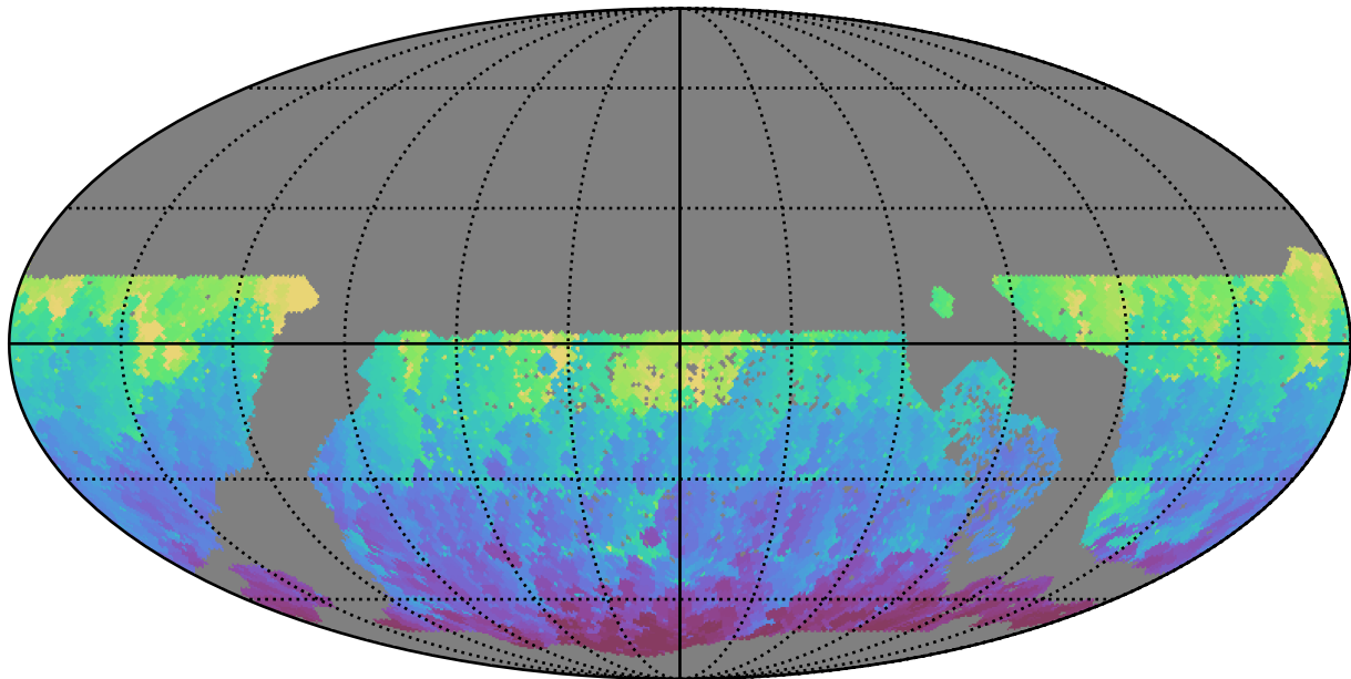
ddf_acor_sf30_lsf40_lsr50_v3.4_10yrs WFD g band: Min HA
